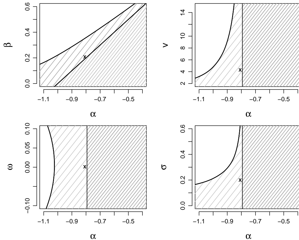
Figure 6: Parameter region and parameter estimate obtained for the Student's t location model and applied to the U.S. consumer price index time series from January 1947 to February 2016.
