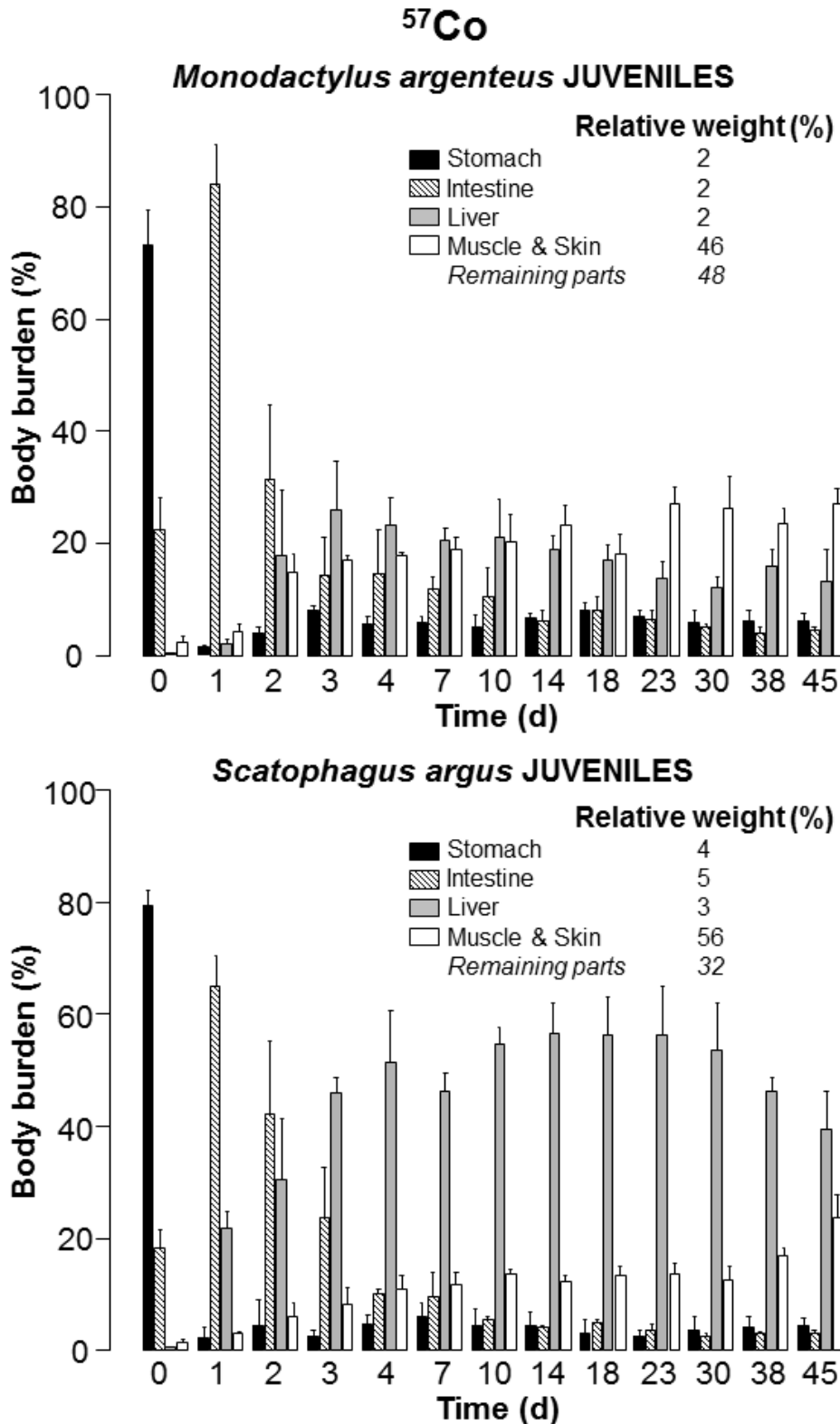
Figure 2. ^{57}\text{Co} distribution among 4 body compartments (intestine, stomach, liver, and muscles with skin) of juvenile silver moony ( M. argenteus ) and spotted scat ( S. argus ) over the depuration phase after feeding with radiolabelled brine shrimp. At each time three fish were dissected. All the values are expressed as percentage of the whole-body activity (means + SD).
