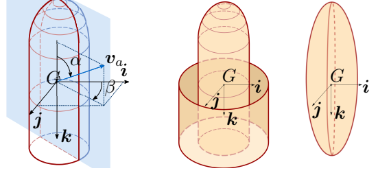
Figure 2. The (\alpha, \beta) angles.
