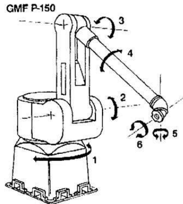
Figure 25. The GMF P150 robot.
