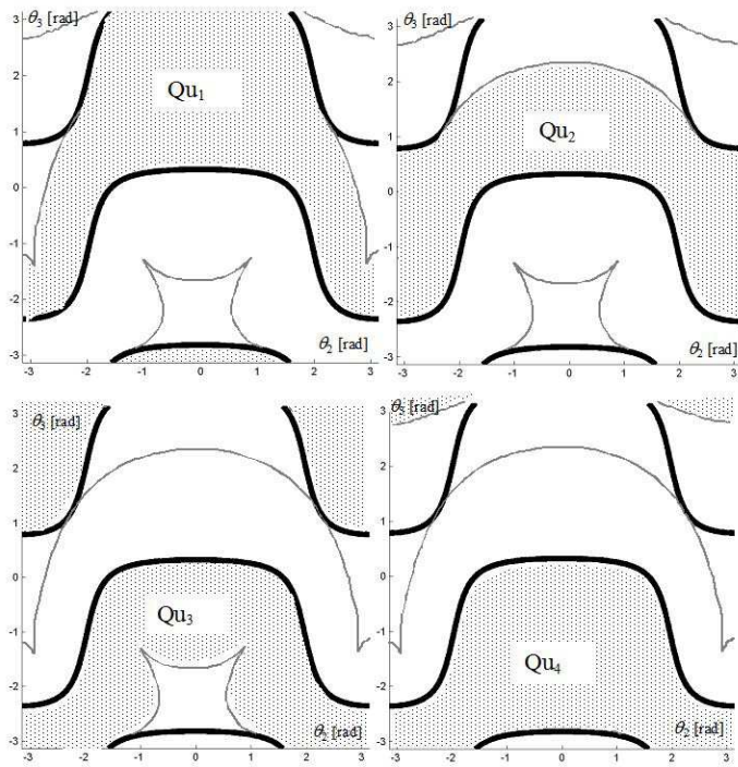
Figure 17. The four uniqueness domains for the robot of Figure 1.
