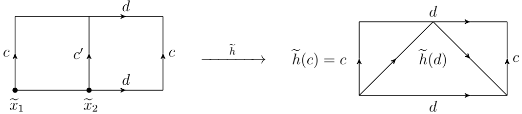
FIGURE 2. A lift \tilde{h} to T of the homeomorphism h .
