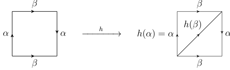
FIGURE 1. The homeomorphism h of K .
