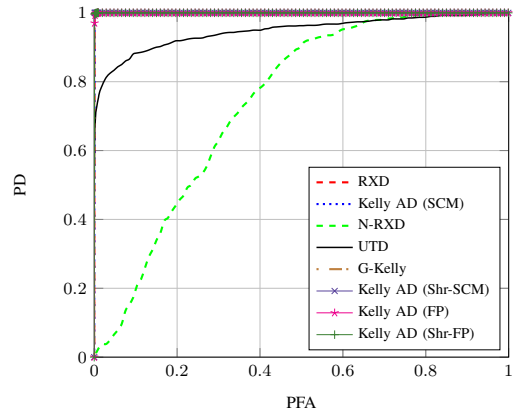
Fig. 9: ROC curve comparing the different detectors in Gaussian environment ( m = 6 , N = 24 and SNR=10 dB).
