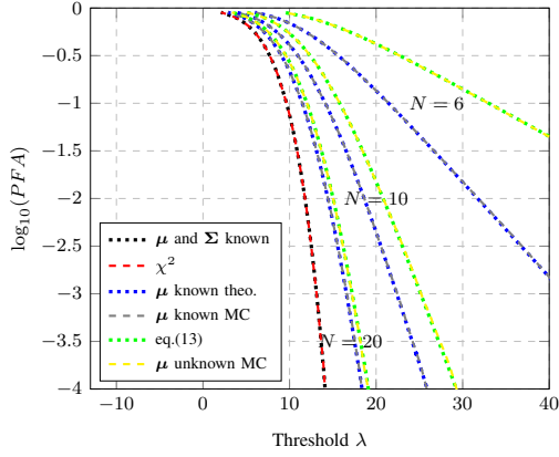
Fig. 1: PFA versus threshold for the \Lambda_{Kelly AD} ( m = 5 ) when (1) \mu and \Sigma are known (Mahalanobis) (red and black curves) (2) only \mu is known (gray and blue curves) (3) Proposition II.1: both \mu and \Sigma are unknown (yellow and green curves).
