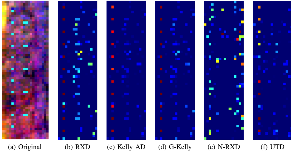
Fig. 7: Conventional Anomaly Detection for artificial targets in real HSI ( m = 6 , N = 24 , same PFA=10^{-1} ).
