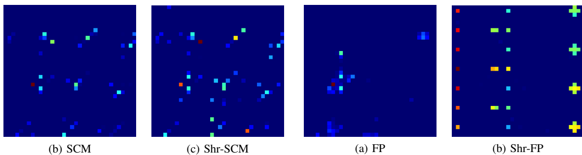
Fig. 11: Extended Kelly AD built with conventional and robust estimates for artificial targets in real HSI ( m = 126 , N = 288 , same PFA=10^{-1} ).
