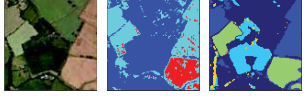
(a) Analysis window. (b) Detection by EM [20, 21]. (c) Detection by DPM-MRF (this paper). Fig. 1. Objects detected in the image (a) using EM (b) and DPM-MRF (c).
