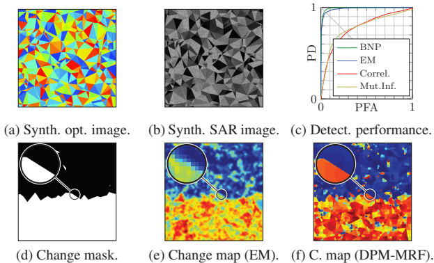
Fig. 2. Change detection on synthetic heterogeneous images.
