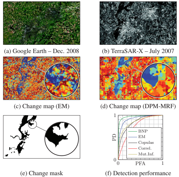
Fig. 3. Change detection results on heterogeneous images
