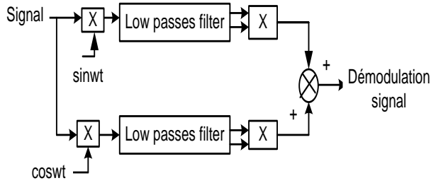
Fig.14. Principe of the demodulation
