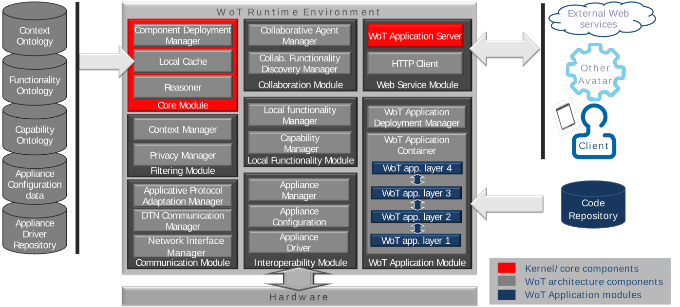
Fig. 2. Web architecture of avatar agents
