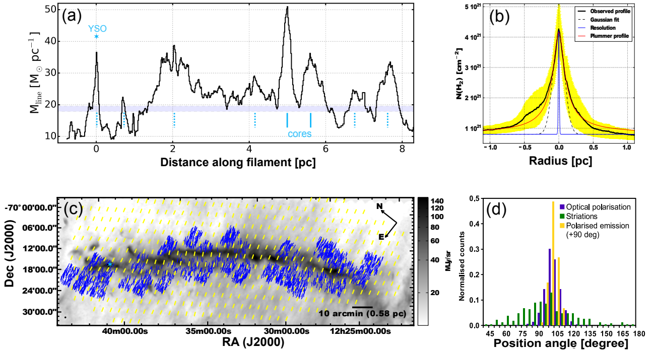
Fig. 4. a) Mass per unit length, M_{\text{line}} ( M_{\odot} \text{pc}^{-1} ), along the main filament derived as explained in Sect. 2.3. The light gray area indicates M_{\text{line,crit}} = 17.9\text{--}19.6 M_{\odot} \text{pc}^{-1} . For illustration, the positions of the YSO (Sect. 3) and the cold dense cores studied by Juvela et al. (2010, 2011) are indicated (solid vertical line markers). Several other sharp peaks seen in the M_{\text{line}} graph are related to candidate dense cores (dotted vertical line markers). b) Radial column density profile perpendicular to the major axis of the filament and averaged along its length. The yellow area shows the dispersion along the filament length. The red and dashed curves show the best Gaussian and Plummer function fits (see Sect. 2.3). The inner blue curve corresponds to the 18.2'' beam resolution of the column density maps. c) POS orientations of the magnetic field as derived from starlight polarization (blue lines, Pereyra & Magalhães 2004) and polarized dust 850 \mu\text{m} emission observed by Planck at 9.6' angular resolution (yellow lines of arbitrary length, Planck Collaboration Int. XXXIII 2016) overlaid on the SPIRE 250 \mu\text{m} map. Equatorial north-east directions are indicated by the compass (corresponding to a rotation of 55° counter-clockwise with respect to north is up). The angular and spatial scales are indicated by the horizontal line in the bottom panel : 10' is equivalent to 0.58 pc. d) Distributions of position angles for low-density filaments/striations (green), optical polarization vectors (blue), and polarized emission vectors (rotated by +90° to trace the POS magnetic field direction; yellow).
