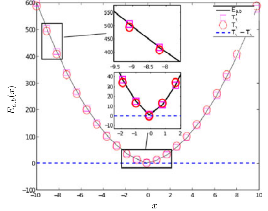
Fig. 1. The potential energy E_{a,b} (solid black line) in (19) ( a = 10 , b = 5 ) and its discretizations using the modified leapfrog schemes T'_s (squares) and T''_s (circles), as well as the difference between the two discretizations T''_s - T'_s (dashed blue line).
