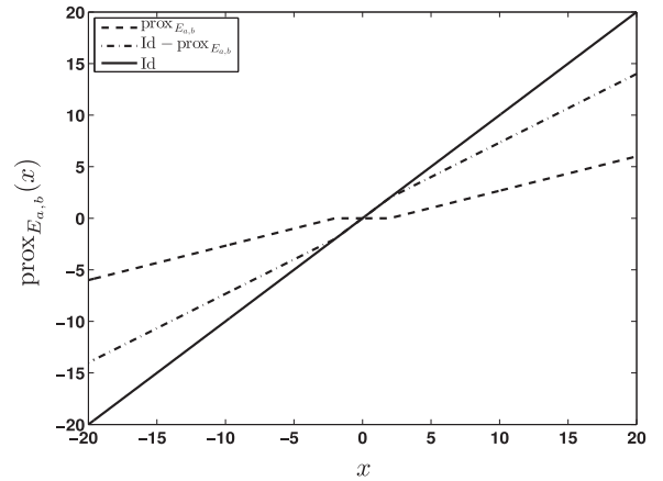
Fig. 2. The proximity operator \text{prox}_{E_{a,b}} , the identity function (Id) and the difference \text{Id} - \text{prox}_{E_{a,b}} for a = b = 2 .
