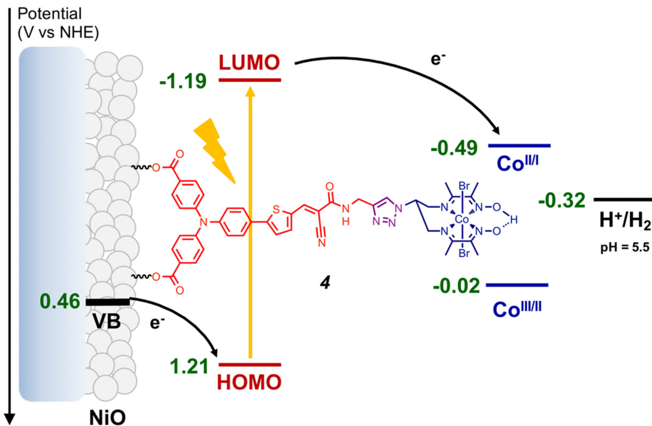
Figure 1. Energy diagram and working principle of the p-type photocathode based on 4 at pH 5.5. The NiO valence band edge potential at this pH value was estimated from the 0.37V vs NHE value determined at pH 7 in ref. 17.
