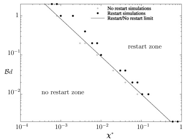
Figure 8 Combined effects of thixotropy and compressibility for the restart of the weakly compressible flow in a pipeline filled with a viscoplastic and thixotropic material (from Wachs et al. (2009)). The Bingham number is set to a value larger than the classical restart limit. \chi^* and Bd are dimensionless numbers for compressibility and thixotropy, respectively.
