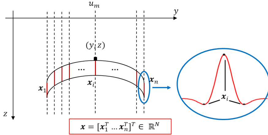
Figure 1: Sampling process for the vector x : red lines represent the samples along the different columns of the image, which are then assembled in the vector x . Only three values are sampled per column to limit the size of the data vector, the latter being the central and two peripheral peak values.
