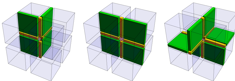
Figure 4.4: Examples of 1-surfaces.
