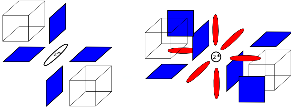
Figure 5.11: Example of \beta_{\mathfrak{H}_1}^{\square}(z^*) in the 3D case. On the left, z^* \in \mathbb{H}_1^3 ( \beta_{\mathfrak{H}_1}^{\square}(z^*) is then the union of the blue faces), and on the right, z^* \in \mathbb{H}_0^3 ( \beta_{\mathfrak{H}_0}^{\square}(z^*) is then the union of the blue and red faces).
