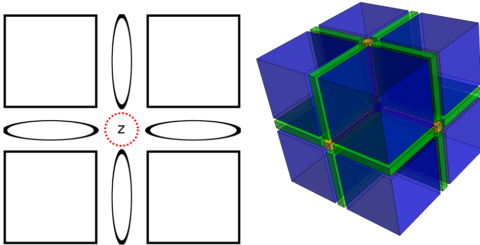
Figure 5.2: The subspace |\beta^\square(z)| we are working in to study AWCness (2D/3D cases).
