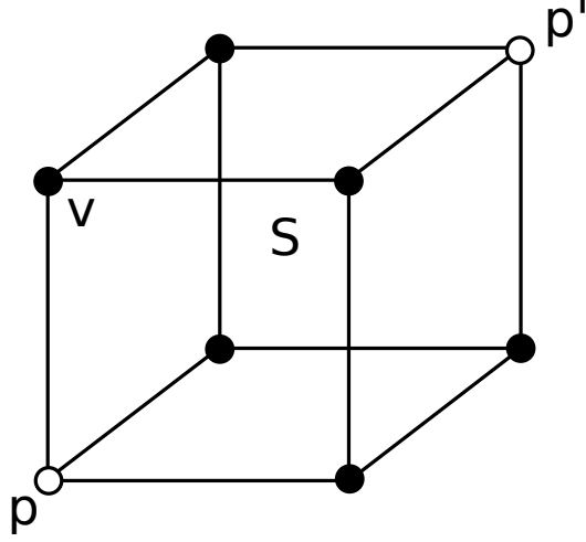
Figure 6.8: \mathcal{H}_n(p) \wedge \mathcal{H}_n(p') \in \alpha(\mathcal{H}_n(p) \wedge \mathcal{H}_n(v)) .
