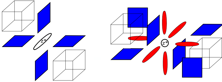
Figure 6.10: Example of \beta_{\mathfrak{H}^1}^{\square}(z^*) in the 3D case. On the left, z^* \in \mathbb{H}_1^3 ( \beta_{\mathfrak{H}^1}^{\square}(z^*) is then the union of the blue faces), and on the right, z^* \in \mathbb{H}_0^3 ( \beta_{\mathfrak{H}^1}^{\square}(z^*) is then the union of the blue and red faces).
