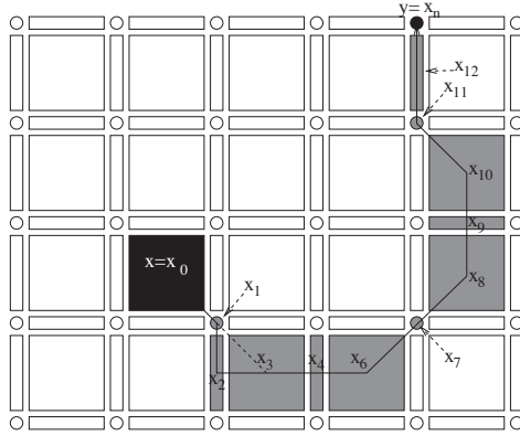
Figure 3.8: A path in \mathbb{H}^2 [11] (p.34)
