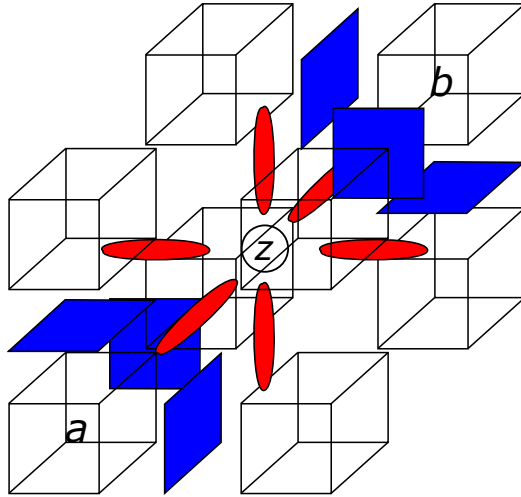
Figure 4.9: Structure of \beta_{\mathfrak{H}^n}^\square(z) when we have (n - \dim(z)) = 3 assuming that |\beta_{\mathfrak{H}^n}^\square(z)| is not connected.
