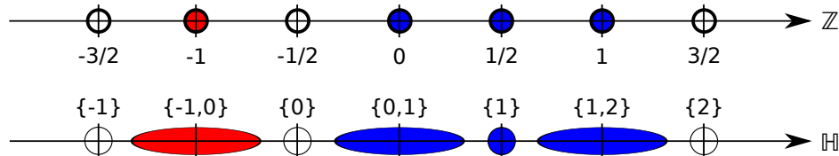
Figure 5.2: Topological isomorphism between |\mathbb{H}^1| and ((\mathbb{Z}/2), \mathcal{U}_{(\mathbb{Z}/2)})
