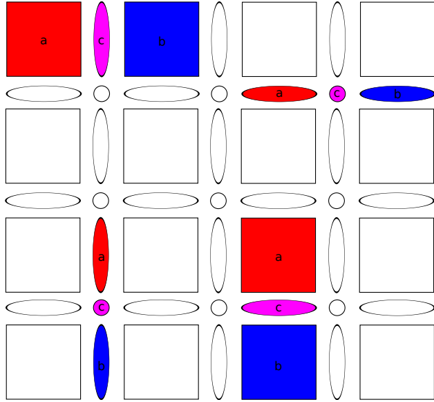
Figure 5.14: Examples of opposites in \mathbb{H}^2 .
