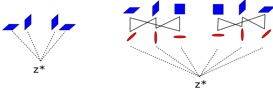
Figure 5.12: Hasse diagrams of |\beta_{\mathfrak{H}}^{\square}(z^*)| of Figure 5.11. On the left, z^* \in \mathbb{H}_1^3 and |\beta_{\mathfrak{H}}^{\square}(z^*)| is an union of two disjoint 0-surfaces. On the right, z^* \in \mathbb{H}_0^3 and |\beta_{\mathfrak{H}}^{\square}(z^*)| is an union of two disjoint 1-surfaces.
