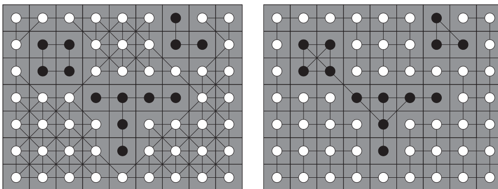
Figure 3.6: u_{\text{bin}} [11] (p. 31) supplied with the (4, 8) -topology on the left and with the (8, 4) -topology on the right (the foreground is in black and the background in white).
