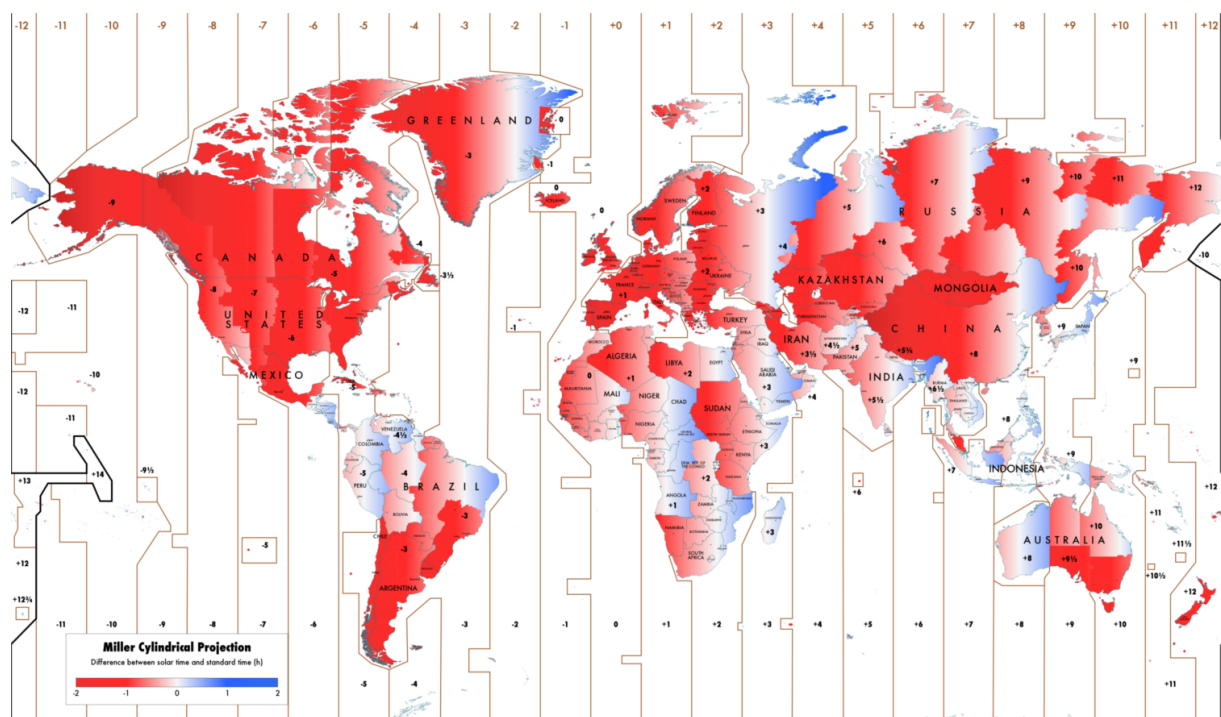
Figure 4: World Map of Solar Time vs. Daylight Savings Time (adapted from [36]). Areas in strong red are two hours or more behind local solar time and are likely to benefit similarly from a change in (local) summer time zone.
