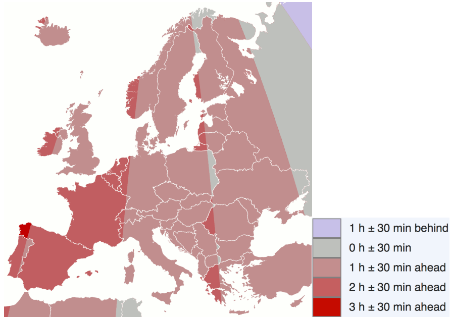
Figure 1: Difference between legal time and local mean time in Europe during the summer [25].
