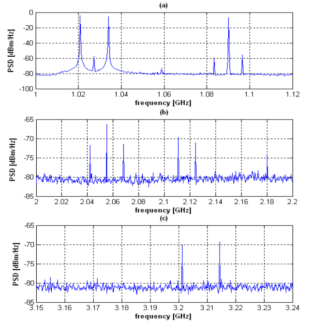
Fig. 1. (a) Fundamental frequencies of a 3-tone signal with frequencies at 1.021 GHz, 1.034GHz and 1.09GHz. (b) Weak 2 nd harmonics. (c) Weak 3 rd harmonics.
