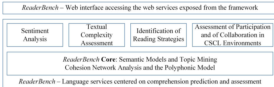
Figure 2. ReaderBench architecture.
