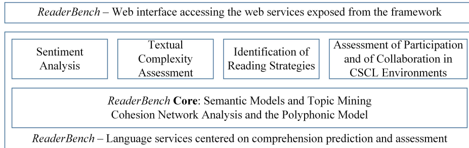
Figure 2. ReaderBench architecture.
