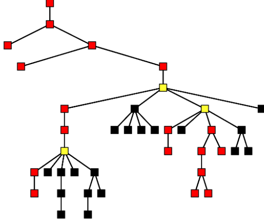
Figure 2: Spectral decomposition of a 40–vertex tree at \lambda = 1 : \mathbb{S}_1 (in red) consists of 5 connected components, and its boundary \partial\mathbb{S}_1 (in yellow) has size 3, so the multiplicity of 1 is 5 - 3 = 2 .
