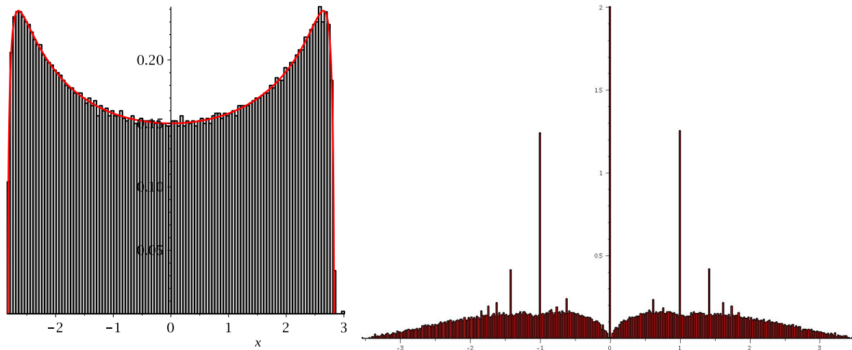
Figure 1: Left: histogram of the eigenvalues of a uniform 3-regular random graph on n = 10^4 vertices (in gray), compared with the Kesten McKay density (3) (in red). Right: histogram of the eigenvalues of the Erdős-Rényi random graph with n = 10^4, p = 2/n . One of the main motivations for our work is to relate this striking difference of regularity to the geometry of the graphs.
