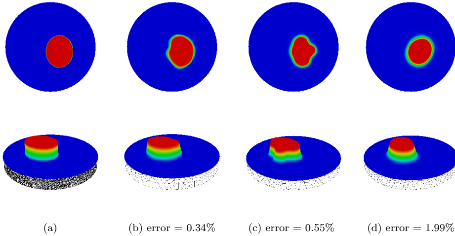
Figure 11 – Reconstruction of an ellipse by using the AEI method: (a) Exact coefficient \Re(\kappa_{ex}) . (b) Reconstructed permittivity \Re(\kappa_{L_4}^{(4)}) with 2%-noisy data and \delta = 5.10^{-3} . (c) Reconstructed permittivity \Re(\kappa_{L_4}^{(4)}) with 5%-noisy data and \delta = 1.10^{-2} . (d) Reconstructed permittivity \Re(\kappa_{L_4}^{(4)}) with 10%-noisy data and \delta = 5.10^{-2} .
