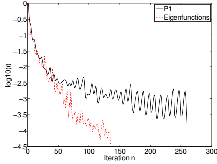
Figure 7 – Convergence of the BFGS minimization algorithm (Step 1 of the AEI method): decrease of the gradient norm.
