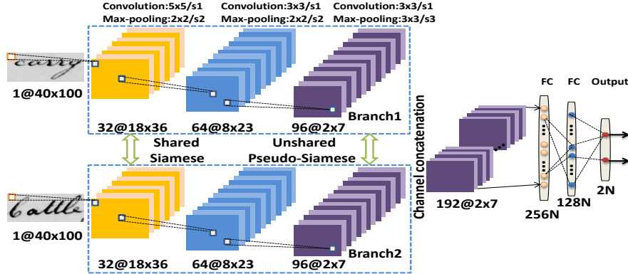
Figure 3. Overview of Siamese and pseudo-Siamese classification network models.
