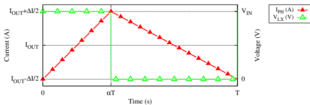
Fig. 8 Current and voltage waveforms for a 1-phase buck converter in CCM
