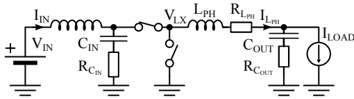
Fig. 7 1-phase buck converter with parasitic elements on passive components.
