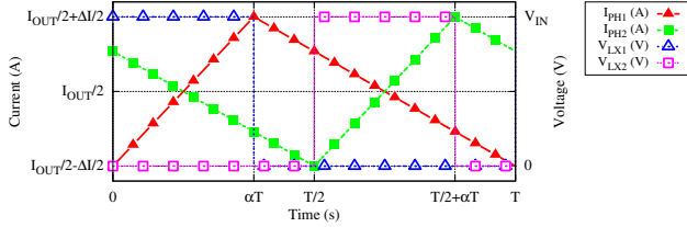
Fig. 10 Current and voltage waveforms for a 2-phase buck converter in CCM.
