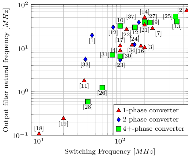
Fig. 1 Output filter natural frequency versus switching frequency.
