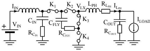
Fig. 12 3-level converter with parasitic elements on passive components.
