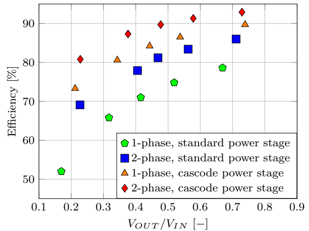
Fig. 17 Post-layout efficiency of active components of converters
