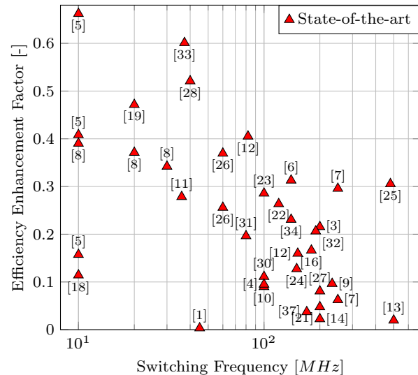
Fig. 3 Efficiency Enhancement Factor versus switching frequency.
