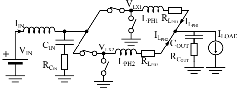
Fig. 9 2-phase buck converter with parasitic elements on passive components.
