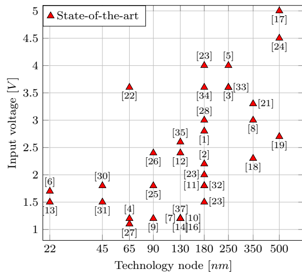
Fig. 6 Input voltage versus technology node.
