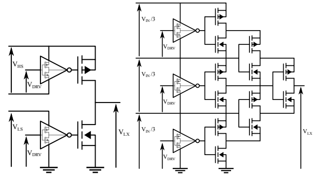
Fig. 16 Standard (left) and cascode (right) power stage.
