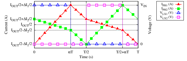
Fig. 11 Current and voltage waveforms of a 2-phase coupled buck converter in CCM.
