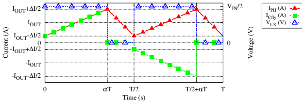
Fig. 13 Current and voltage waveforms for a 3-level buck converter in CCM.
