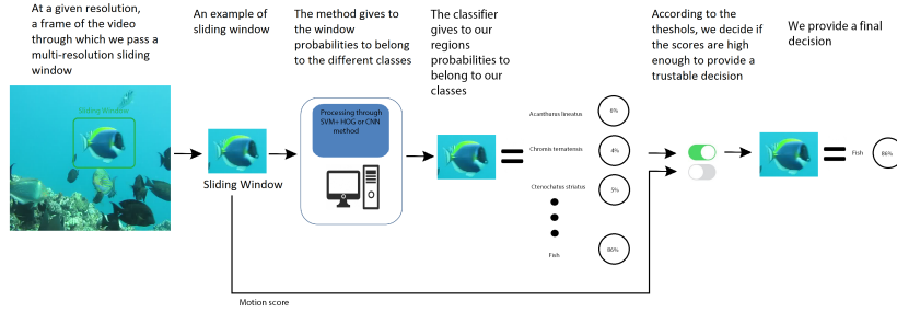
Fig. 3. Detection/Recognition pipeline
