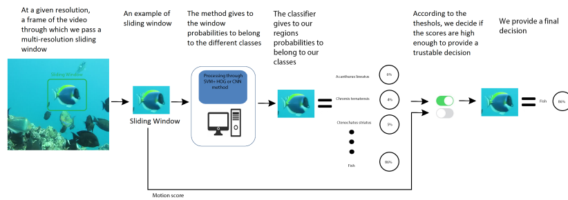
Fig. 3. Detection/Recognition pipeline
