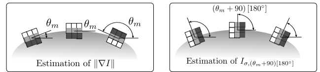
Figure 2: Positions of the steerable filters at the level of the edges to build the gradient image \|\nabla I\| and image derivative I_{\sigma, (\theta_m + 90^\circ) [180^\circ]}(x, y) .
