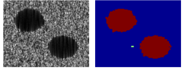
Fig. 9. Estimated TRF (left) and label map (right) for a two-class image with K = 3 (ISNR = 14.46 and OA = 0.8).
