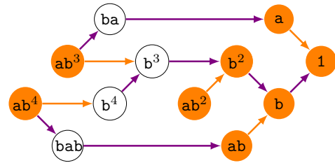
■ Figure 10 The minimal Garside family of the monoid \mathbf{BS}^+(3, 2) from Example 20.
