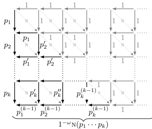
■ Figure 4 Proof of Lemma 10: the normal forms of those \mathcal{Q} -words inducing a same action coincide.
