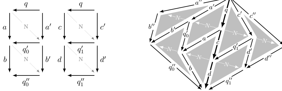
■ Figure 5 Proof of Proposition 11: initial data (left) can be pasted into Condition (◆) (right).
