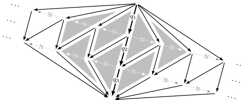
■ Figure 3 From an initial \mathcal{Q} -word q_1q_2q_3 , one applies normalisations on the first or the second 2-factors alternatively up to stabilisation, beginning on the first 2-factor q_1q_2 (on the right-hand side here) or on the second q_2q_3 . The gray zone corresponds to Condition (\blacklozenge) as defined in Definition 6.
