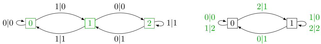
■ Figure 2 Two (dual) Mealy automata: the left-hand one computes the division by 3 in base 2 (most significant digit first) vs the right-hand one computes the multiplication by 2 in base 3 (least significant digit first).
