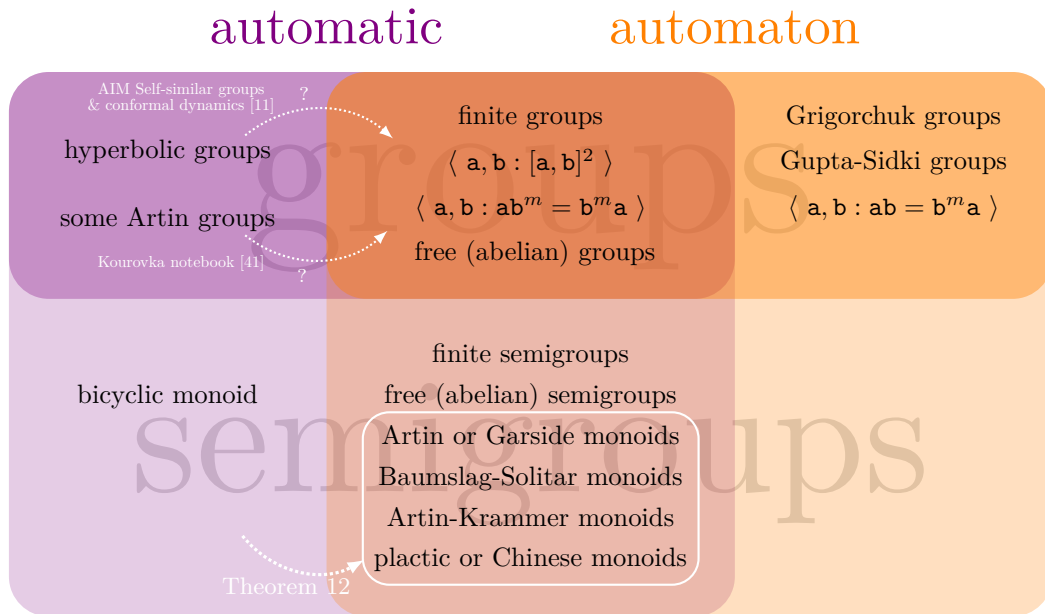
■ Figure 1 The big picture: comparing the classes of automatic vs automaton (semi)groups.
