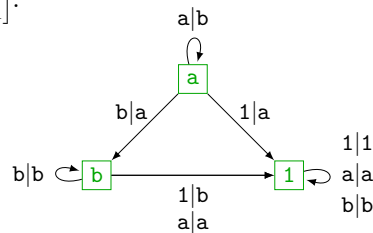
■ Figure 8 The Mealy automaton associated with the monoid \langle a, b : ab = a \rangle^+ from Example 18.
