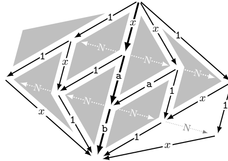
■ Figure 7 Computing the breadth (3, 4) for the bicyclic monoid \mathbf{B} from Example 17.
