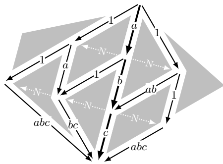
■ Figure 6 Computing the breadth (3, 2) for any finite monoid \mathcal{F} as in Example 16.
