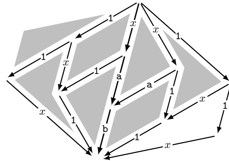
■ Figure 6 Computing the breadth (3, 4) for the bicyclic monoid \mathbf{B} from Example 16.
