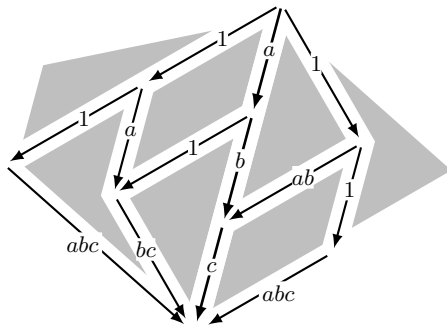
■ Figure 5 Computing the breadth (3, 2) for a finite monoid \mathcal{F} as in Example 15.
