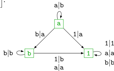
■ Figure 7 The Mealy automaton associated with the monoid \langle a, b : ab = a \rangle^+ from Example 17.
