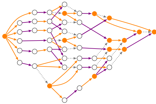
■ Figure 8 The minimal Garside family of the monoid \mathbf{AK}^+ \left( \begin{bmatrix} 1 & 3 & 2 \\ 4 & 1 & 3 \\ 2 & 4 & 1 \end{bmatrix} \right) from Example 18.
