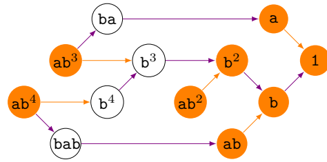
■ Figure 9 The minimal Garside family of the monoid \mathbf{BS}^+(3, 2) from Example 19.
