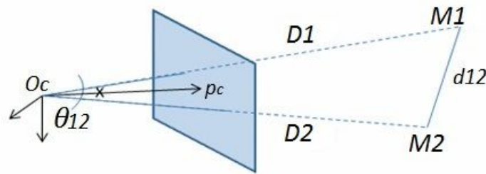
Figure 5. The triangle formed by M_1 , M_2 (3D points in the camera frame) and O_c is shown. d_{12} is the Euclidean distance between M_1 and M_2 that is supposed to be known, and D_1 , D_2 are their depths relative to O_c .
