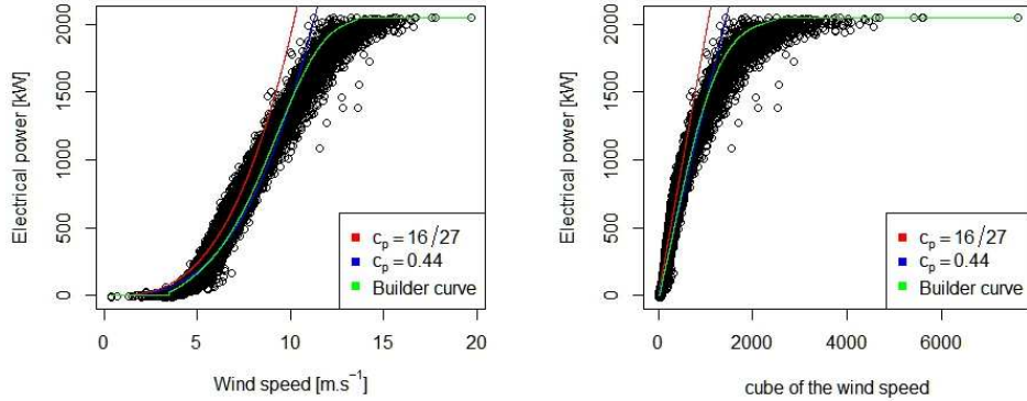
Figure 1: Empirical observations and theoretical power curves for different power coefficient values, compared to the curve provided by the turbine builder.
