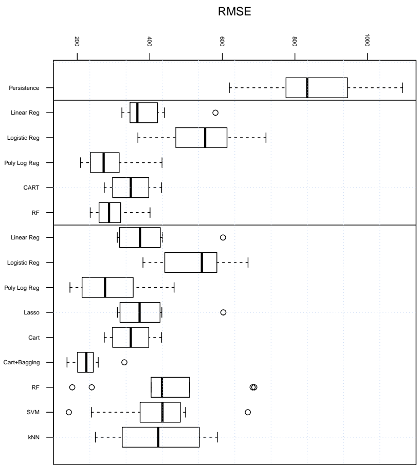
Figure 4: Boxplots of the RMSE for the different procedures using the mean of wind speed measures.
