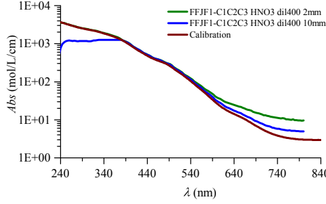
Figure 2: Non destructive determination of the iron oxide concentration by UV-Vis spectroscopy. The spectrum of the sample diluted 400 times in \text{HNO}_3 at \text{pH}\sim 2 (for colloidal stability) is recorded between 240 and 800 nm. The extinction coefficient e(\lambda) calculated after normalization by the light path L (cm) and the equivalent iron concentration ( 1.24 \text{ mol} \cdot \text{L}^{-1} as determined here) is fitted to a calibration curve obtained from measurements on samples at concentrations titrated by atomic emission spectroscopy [29]. Then the weight concentration c_0 = 99 \text{ g} \cdot \text{L}^{-1} is simply deduced by multiplying by 80 \text{ g} \cdot \text{mol}^{-1} ( \sim half the molar mass of \gamma\text{-Fe}_2\text{O}_3 ). The deviation between the experimental spectra and the calibration curve towards large wavelengths is ascribed to a light scattering background (since the nanoparticles are particularly large in this study). The plateau for the larger light path ( L=10 mm) is an artifact due to the lower limit of the detector.
