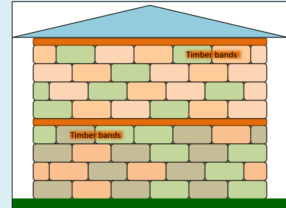
Traditional construction methods throughout many parts of the Himalaya have utilized hand-cut stone blocks with wood spacers, called “timber bands” or “tie beams.” Timber bands tend to isolate smaller portions of a stone wall relative to seismic shaking, thus preventing the entire wall from undergoing catastrophic failure. Timber bands, carved into decorative snakes, are clearly seen in Kathmandu on Hanuman Dhoka Palace (yellow arrows in photo below) in Durbar Square. The old palace experienced far less damage from the Gorkha earthquake than did the newer addition to the palace (white building to the left).
