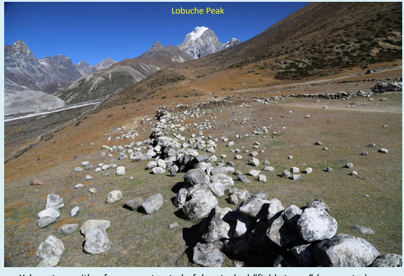
Yak pasture with a fence constructed of dry-stacked “field stones” (no mortar) was toppled during the 2015 Gorkha earthquake sequence. This yak pasture complex is located on the high NE lateral moraine (Khumbu Glacier) between Pheriche and Dughla. Unsupported top-heavy construction, unstable substrate, and possible amplification of ground shaking on the moraine crest all contributed to failure.
