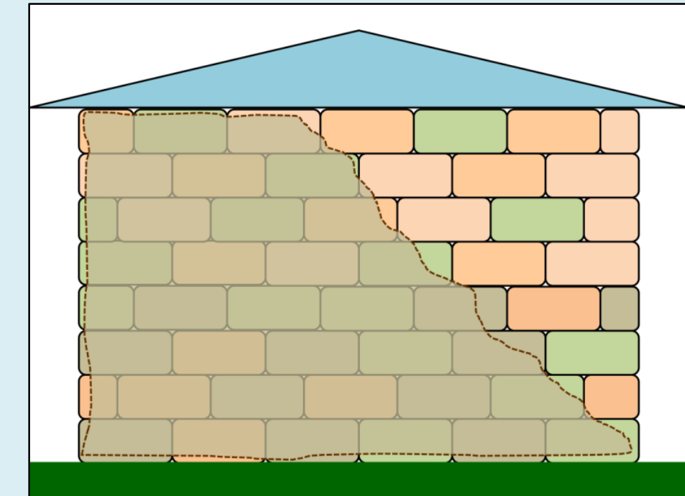
Older, traditional buildings in the Khumbu were constructed of uncut “field stone” with no mortar or external plaster, just small stones placed between larger stone blocks to fill gaps; some buildings used dried mud mortar as an external “plaster”, as shown in the diagram and photo above (Lukla).
