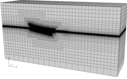
(a) General view of the mesh and the computational domain
