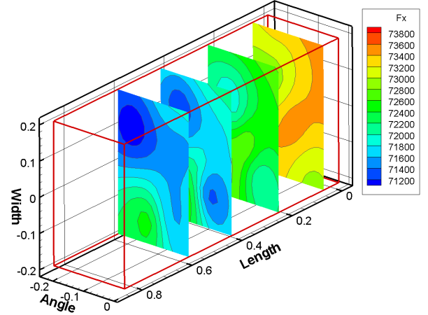
(a) Cutting planes of the response surface
