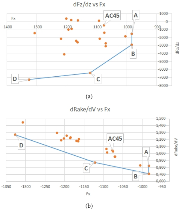
Figure 12: Pareto fronts
