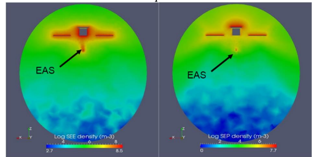
Figure 14. Log of secondary electron (left) and photoelectron (right) density in the X - Z plane
