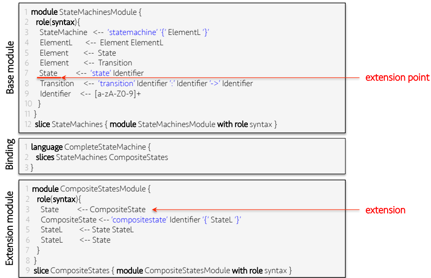
Figure 9: Exogenous extension of language modules in Neverlang
