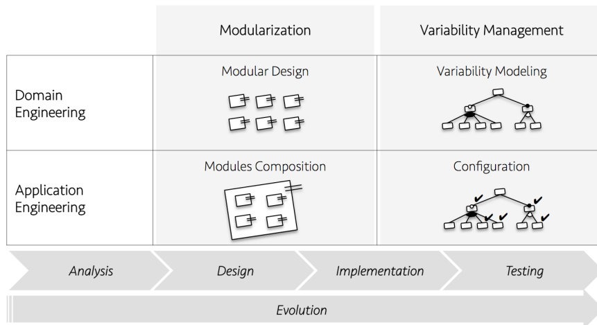
Figure 2: Phases of the SPLE’s life cycle
