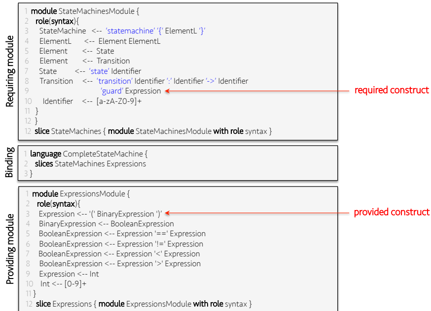
Figure 11: Exogenous aggregation of language modules in Neverlang
