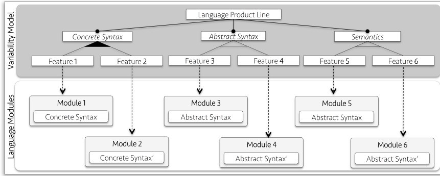
Figure 16: Boolean feature models for representing multi-dimensional variability
