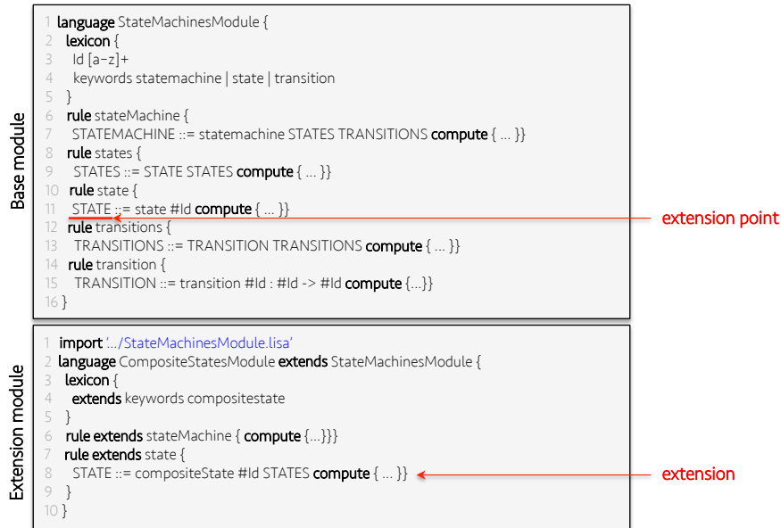
Figure 8: Exogenous extension in LISA
