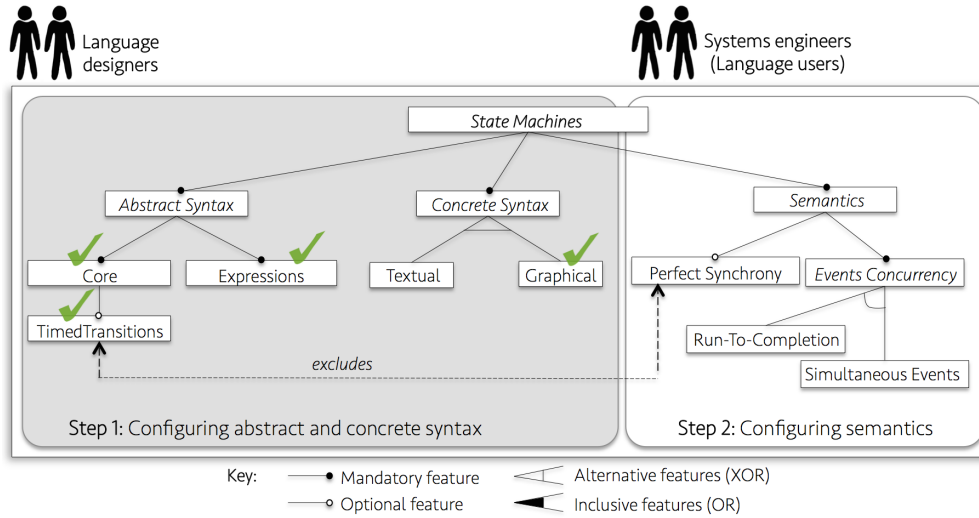
Figure 7: Example for multi-staged configuration of a language product line
