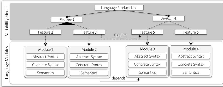
Figure 14: Boolean feature models for representing functional variability
