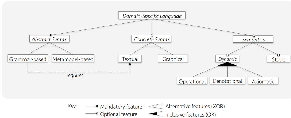
Figure 1: Technological spaces for the implementation of domain-specific languages
