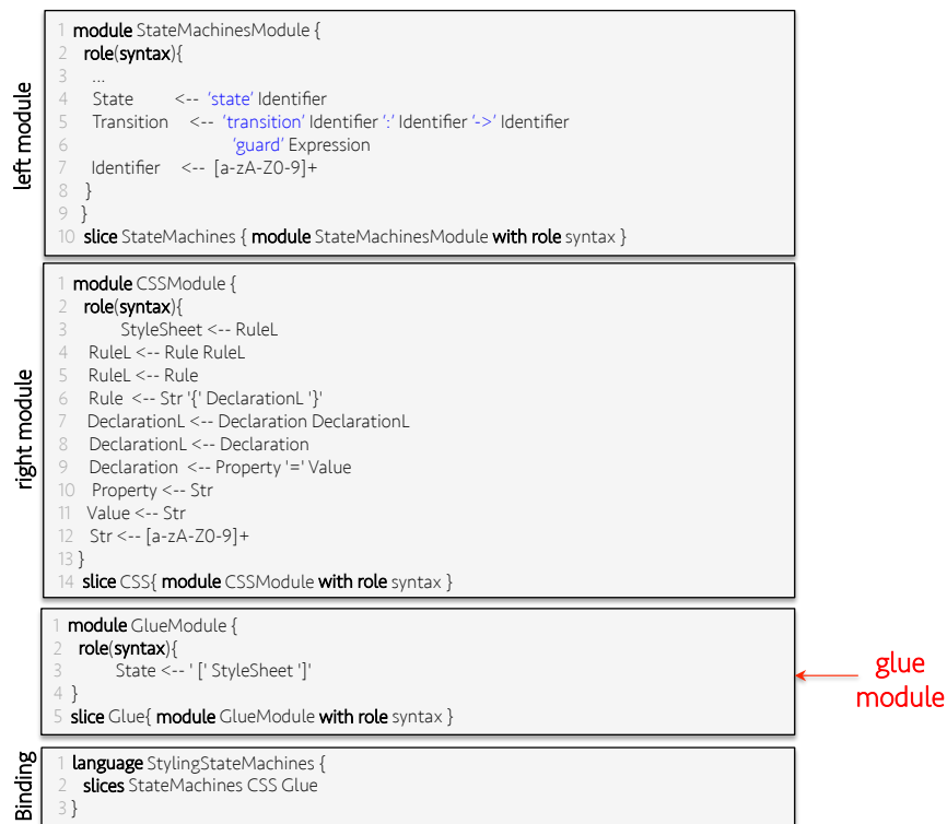
Figure 13: Exogenous unification in Neverlang
