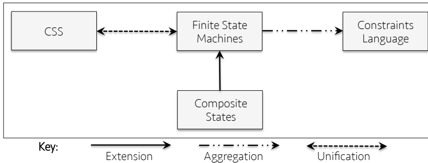
Figure 5: Example of extension composition
