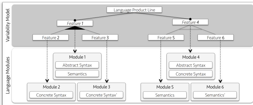
Figure 15: Boolean feature models for representing syntactic and semantic variability
