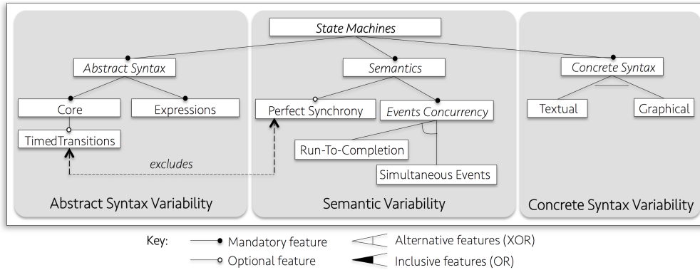
Figure 6: Multi-dimensional variability for a state machine language
