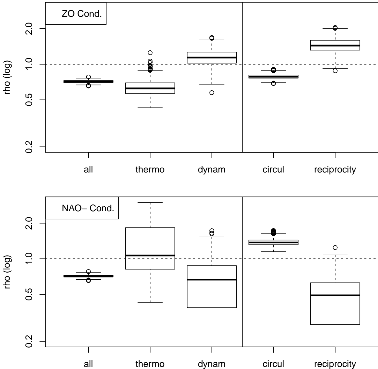
Figure 7. Changes in probability ratios from weather regimes in Weather@Home simulations. The probability ratios (vertical axes) are shown on a logarithmic scale. The horizontal dashed lines show the reference \rho = 1 line. The dynamical contribution is the product of the circulation and reciprocity contributions. The upper panel is the conditional probability ratios for the Zonal regime. The lower panel is for the NAO- regime.
