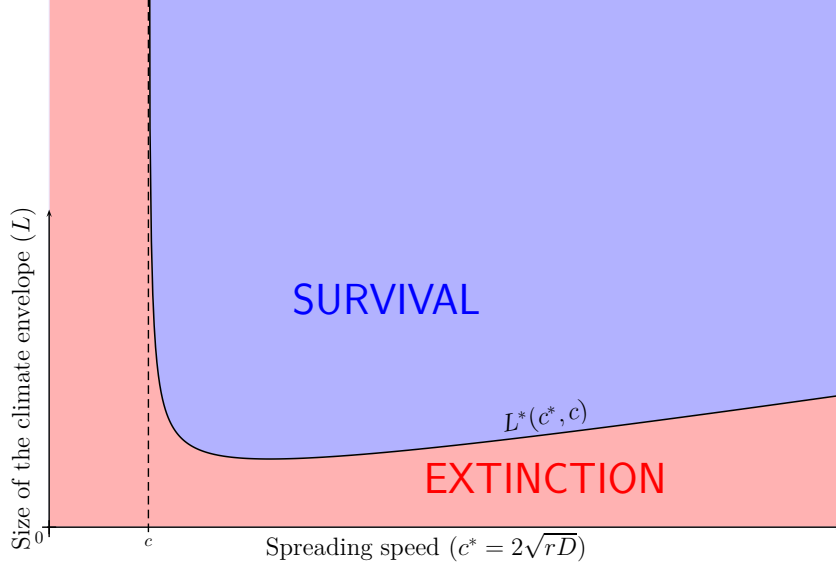
Figure 2: Schematic representation of the behaviour of the population density u as a function of the size of the climate envelope L and the potential spreading speed c^* = 2\sqrt{rD} . Only a population in a wide climate envelope or with a high potential spreading speed can survive climate change.
