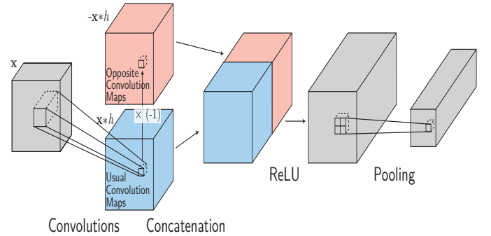
Fig. 1. MaxMin scheme. After the convolutional layer, the resulting maps (in blue) are duplicated negatively (in red). Both stacked maps are concatenated to get the MaxMin output that will pass through the ReLU before pooling.
