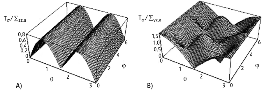
Figure 3. T_\sigma normalized distribution versus (\varphi, \theta) in tension (a) along z and in torsion, (b) (pure shear in the plane (y, z) )
