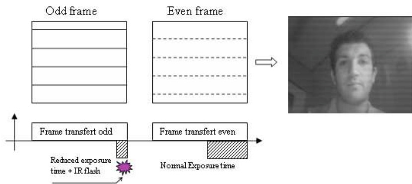
Figure 1. Acquisition Principle
