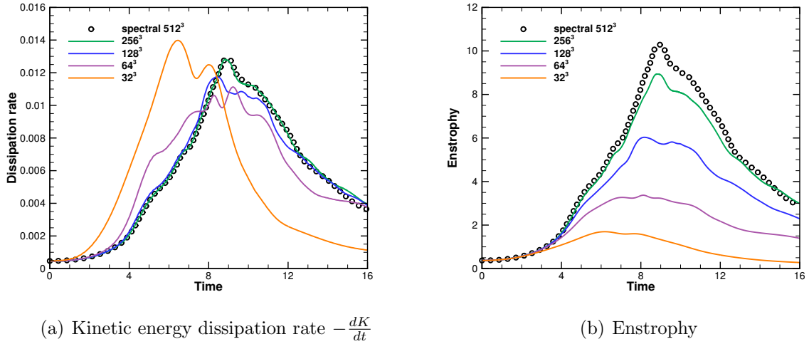
Figure 15: Grid convergence for the kinetic energy dissipation rate and the evolution of enstrophy using the baseline 5 th -order FE-MUSCL scheme.
