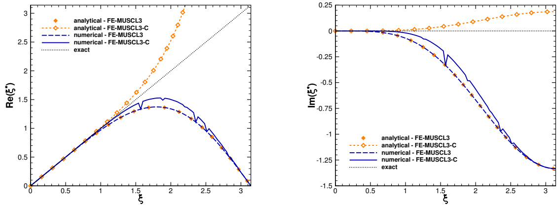
Figure 2: Comparison of numerical spectral analysis with linear analytical theory. Baseline FE-MUSCL3 scheme and with confinement ( \varepsilon = 1.14 k_p ).
