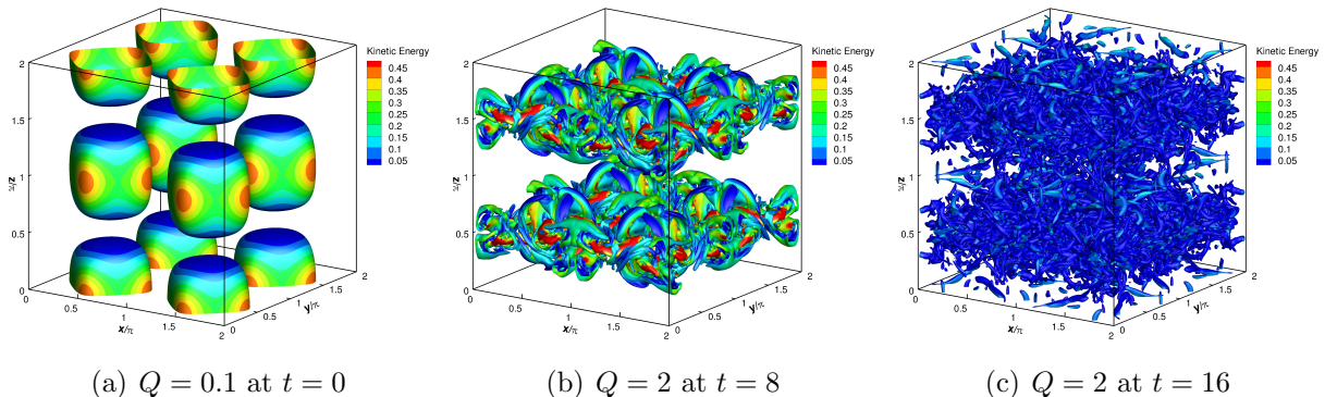
Figure 16: Iso-surfaces of the Q -criterion colored by kinetic energy computed with FE-MUSCL5 and 5^{th} -order Vorticity Confinement on the 256^3 mesh.
