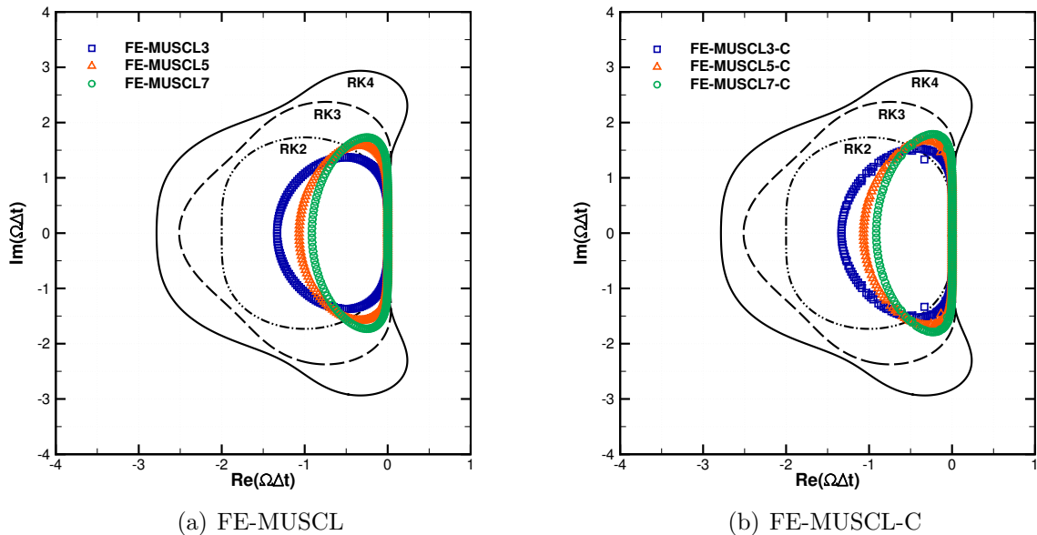
Figure 4: Stability region of classical Runge-Kutta algorithms and Fourier symbol of FE-MUSCL and FE-MUSCL-C space discretizations for \sigma = 1.0 , \varepsilon = 1.14 k_p .
