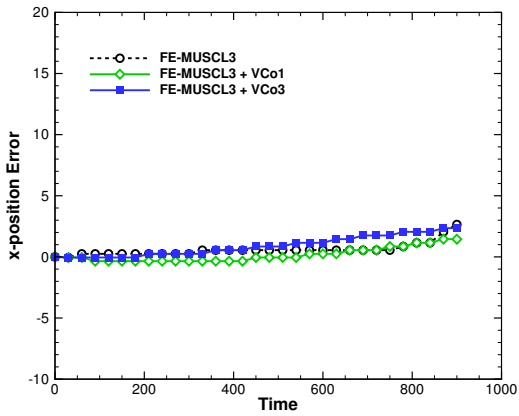
Figure 10: Error in trajectory calculation for the FE-MUSCL3 scheme and VC on the 100^2 mesh.
