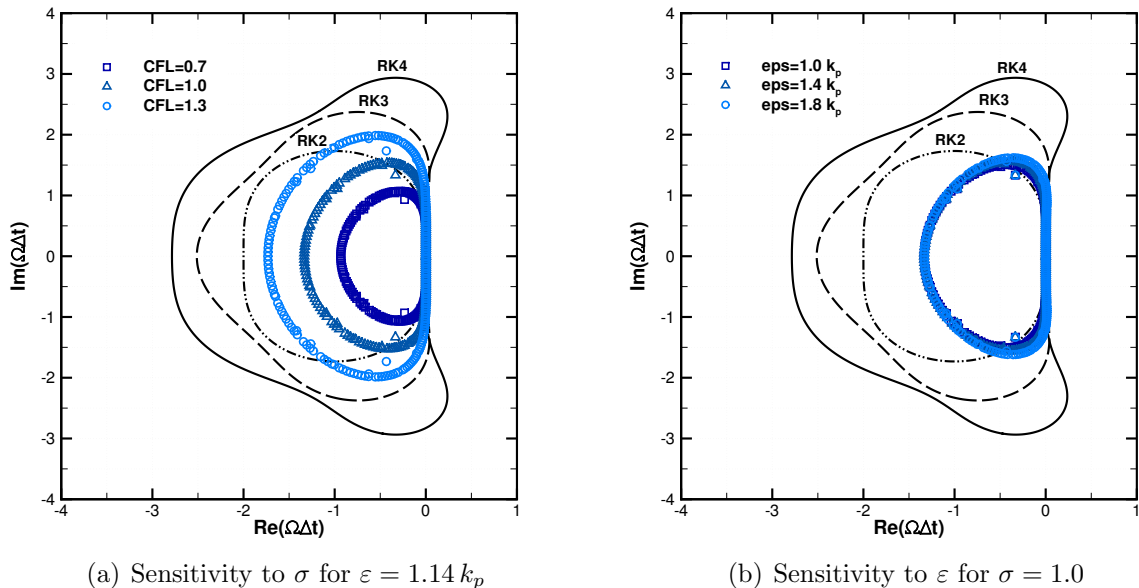
Figure 5: Sensitivity to the value of the CFL number and the confinement parameter for the FE-MUSCL3-C scheme.
