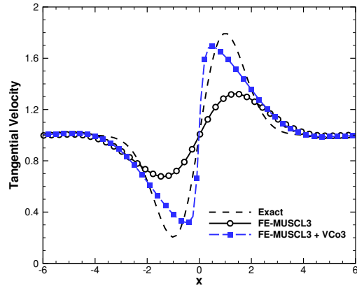
(b) 200^2 mesh
