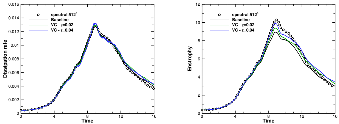
(c) 256^3 mesh
