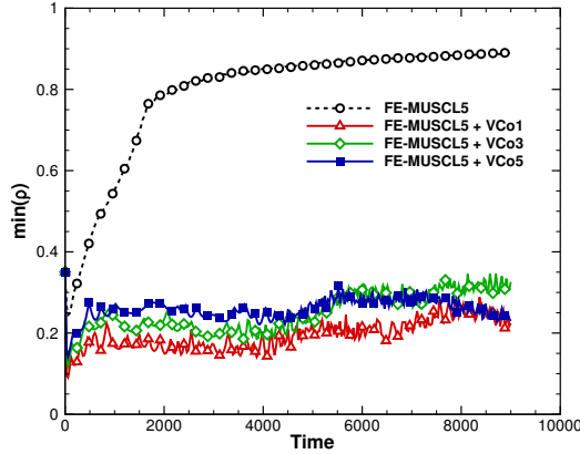
Figure 12: Time evolution of core density using FE-MUSCL5 and VC on the 100^2 mesh.
