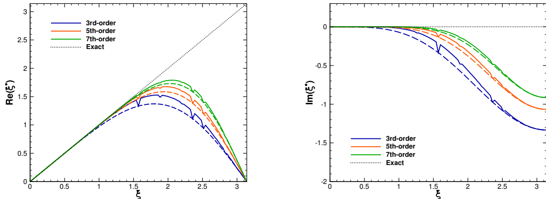
Figure 3: Spectral properties of FE-MUSCL schemes up to 7 th -order. Baseline schemes (dashed lines) and with confinement (solid lines), \varepsilon = 1.14 k_p .
