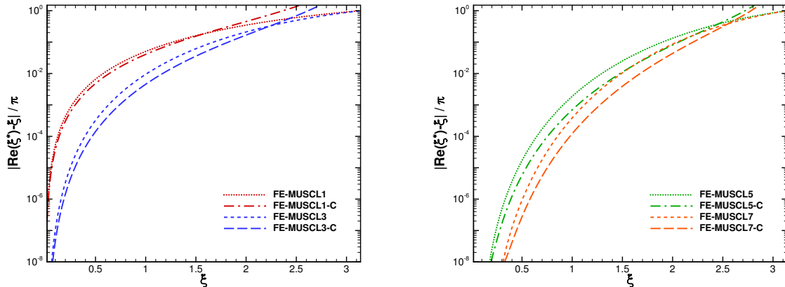
Figure 1: Dispersion error of FE-MUSCL schemes up to 7 th -order with and without confinement for \varepsilon = 1.14 k_p
