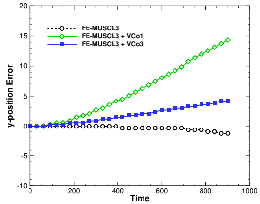
Figure 10: Error in trajectory calculation for the FE-MUSCL3 scheme and VC on the 100^2 mesh.
