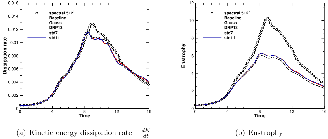
Figure 19: Influence of the velocity gradient calculation scheme. FE-MUSCL5 and 5 th -order Vorticity Confinement, \mu/\varepsilon = 0.4 , \varepsilon = 0.02 , 128^3 mesh.
