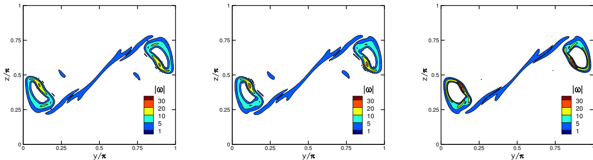
(a) Baseline FE-MUSCL5 - 256^3 mesh (b) FE-MUSCL5 + VC - 256^3 mesh ( \varepsilon = 0.02 ) (c) Spectral - 512^3 mesh
