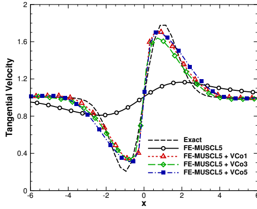
Figure 13: Comparison of tangential velocity profiles after 300 passages across the computational domain ( t = 9000 ) for the FE-MUSCL5 scheme with and without VC on the 100^2 mesh.
