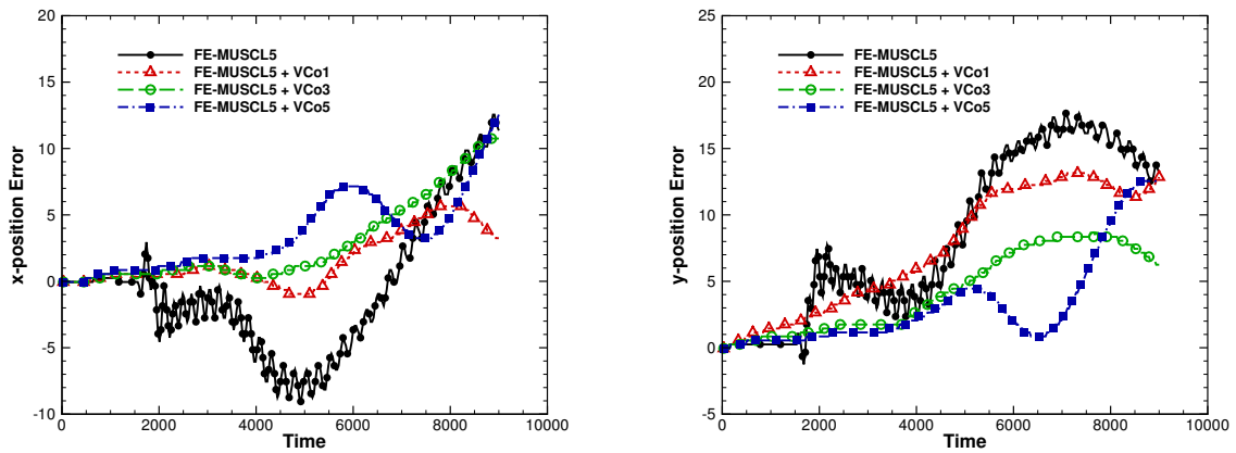
Figure 14: Error in trajectory calculation for the FE-MUSCL5 scheme and VC on the 100^2 mesh.
