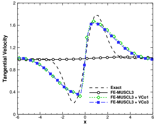
(a) 100^2 mesh
