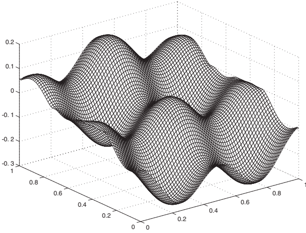
FIG. 6.2. Solution y_\gamma for Example 2 (left) and Example 3 (right) for \gamma = 10^{10} .
