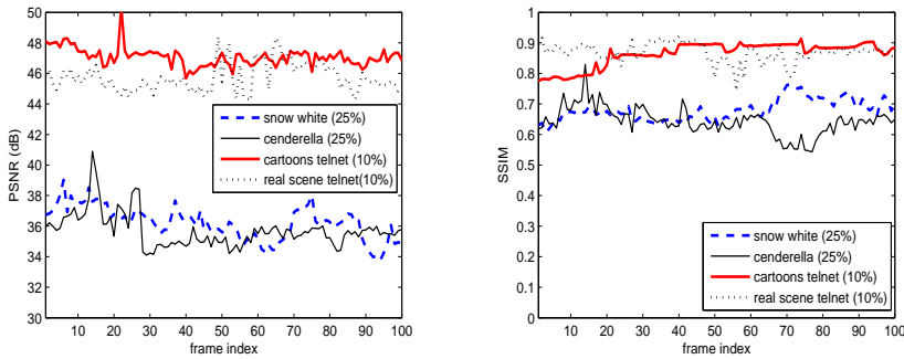
Fig. 8 PSNR and SSIM according to test material and test conditions of Table 2. The embedding pattern is a chess one.
