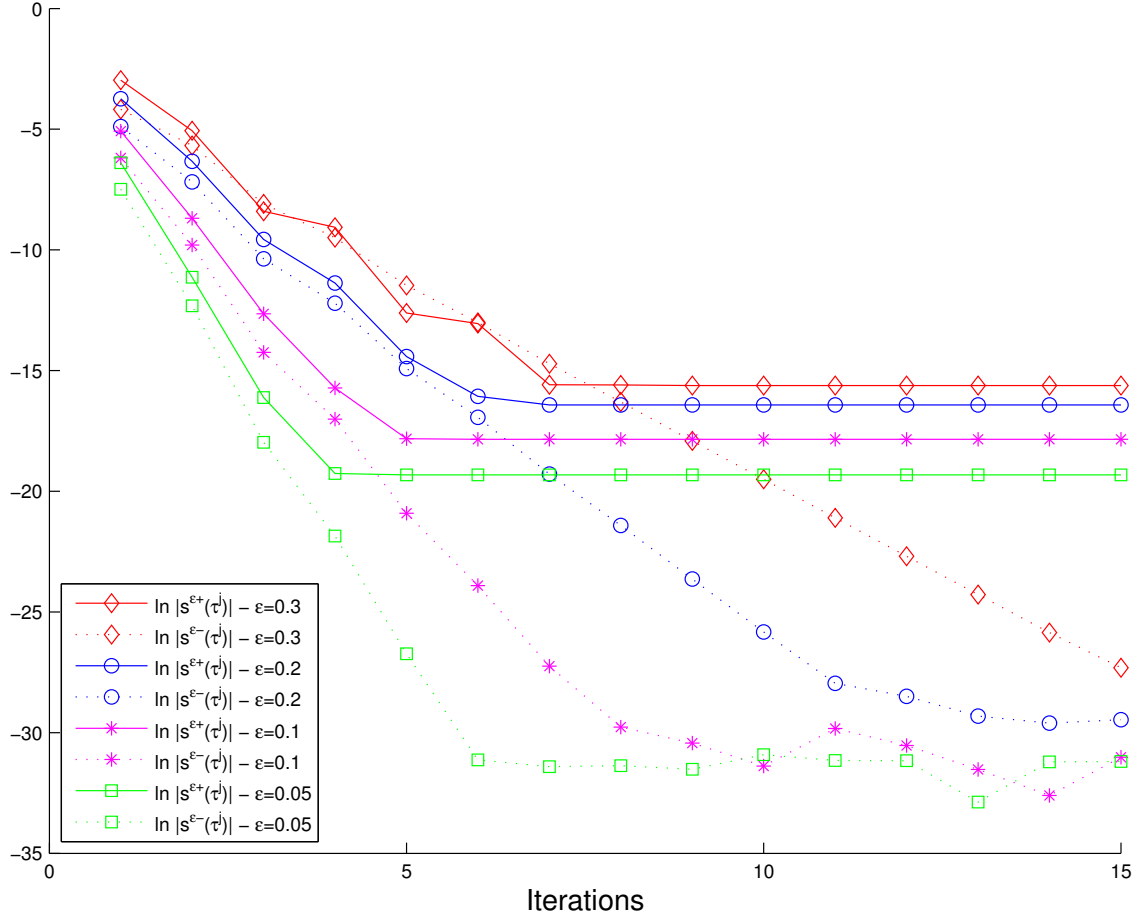
Figure 6: Curves \ln |s^{\epsilon^+}(\tau^j)| and \ln |s^{\epsilon^-}(\tau^j)| with respect to the number of iterations j for several values of \epsilon . The smaller \epsilon , the faster the iterative procedure converges.
