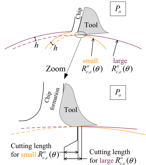
Fig. 10 Illustration of the different contacts between the flank face and the generated surface with respect to radius R_{c,c}^o
